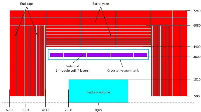
Figure 6.1: 2D layout of CEPC detector magnet (mm)
