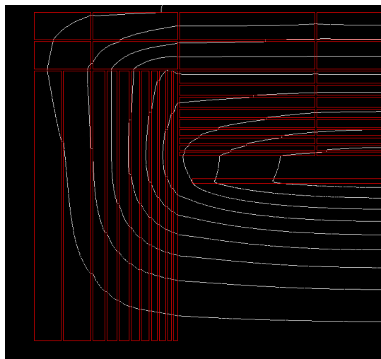
Figure 6.30: Magnetic flux distribution
