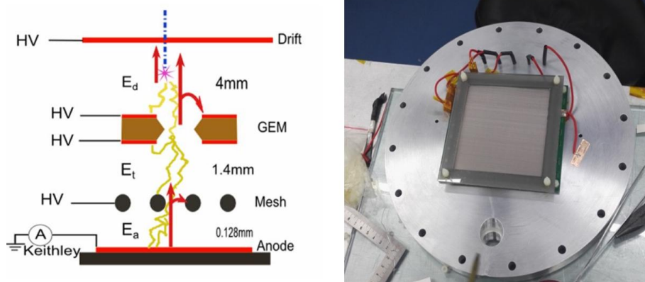
Figure 4.21: Schematic diagram of the detector module.
